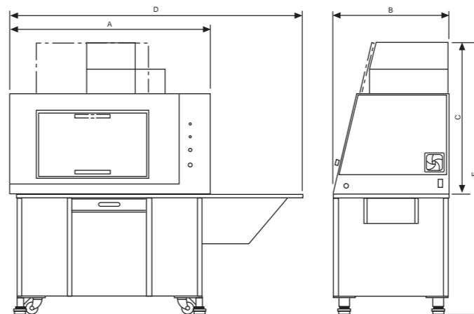
Machine Dimensions.
