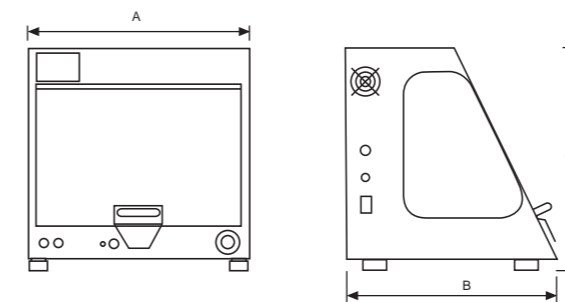
Machine Dimensions.
